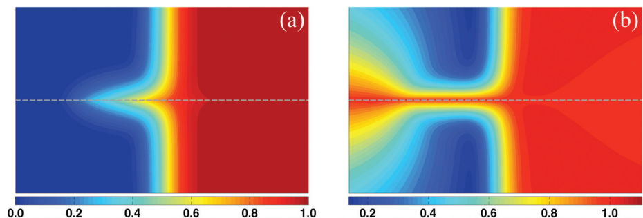
Simulations are performed to study diffusion in a diffusion couple consisting of two components having different hop frequencies to vacant sites. The normalized concentration profile of the component having a larger hop frequency, Fig. (a), shows enhanced diffusion along the grain boundary located horizontally (dashed line) for the case where the hop frequency ratio is 100. The normalized vacancy concentration, Fig. (b), shows its enhancement along the grain boundary, which leads to the higher diffusivity.
