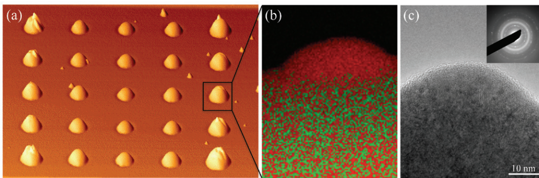
Figs: (a) AFM image of 2-dimensional FIB-fabricated Ga droplet array on GaAs; (b) XEDS cross-sectional map of Ga (red) and As (green) in the vicinity of a Ga droplet shows that the composition of this droplet is pure Ga; (c) cross-sectional TEM image and corresponding diffraction pattern in the vicinity of a Ga droplet indicate that the structure of the Ga droplet is amorphous and there is a polycrystalline GaAs layer underneath the droplet.
