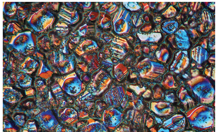
Laura Ligeski, "Secondary Grains of Sintered Barium Titanate"
